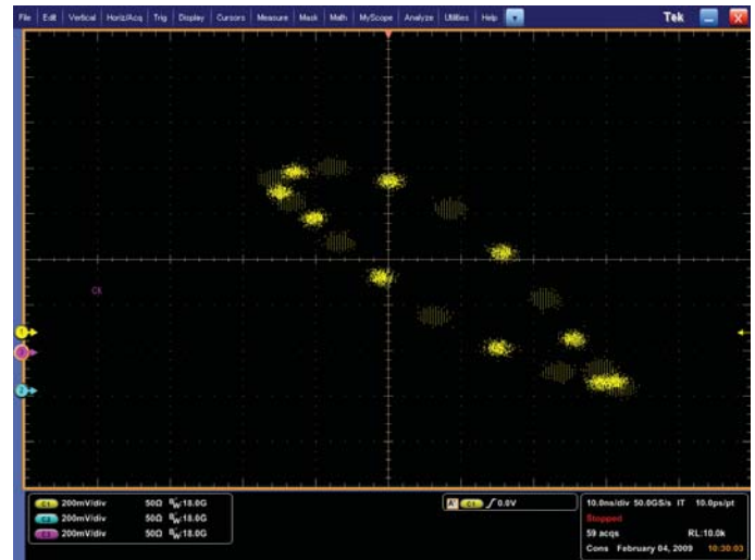
Figure 2b. Two offset clock patterns with Z axis intensity grading.
