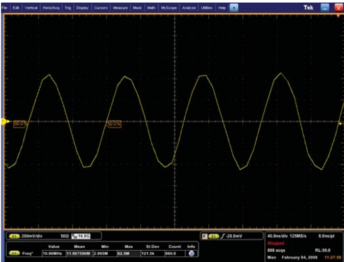
Figure 31a. Undersampling of a 100 MHz sine wave introduces aliasing effects.
