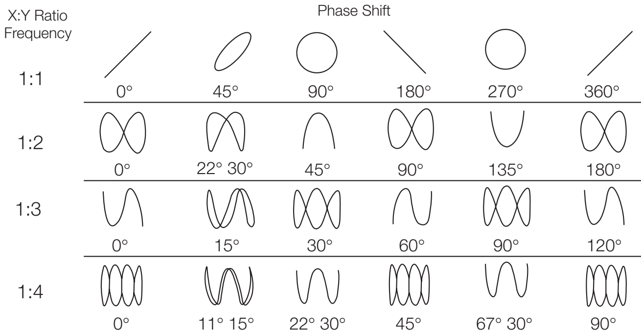
Figure 70. Lissajous patterns.
