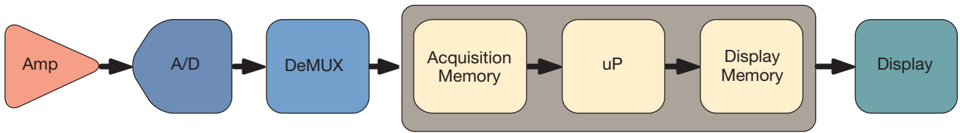
Figure 16. The serial-processing architecture of a digital storage oscilloscope (DSO).
