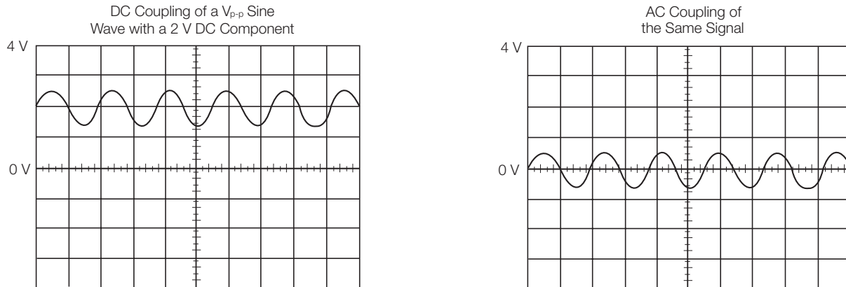
Figure 23. AC and DC input coupling.
