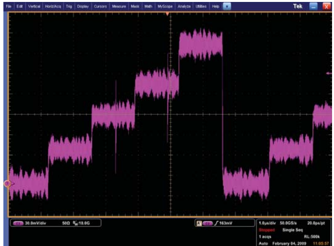
Figure 27. Peak detect mode enables the DPO70000B Series oscilloscope to capture transient anomalies as narrow as 20 ps.
