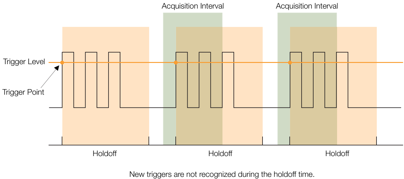
Figure 37. Trigger holdoff.
