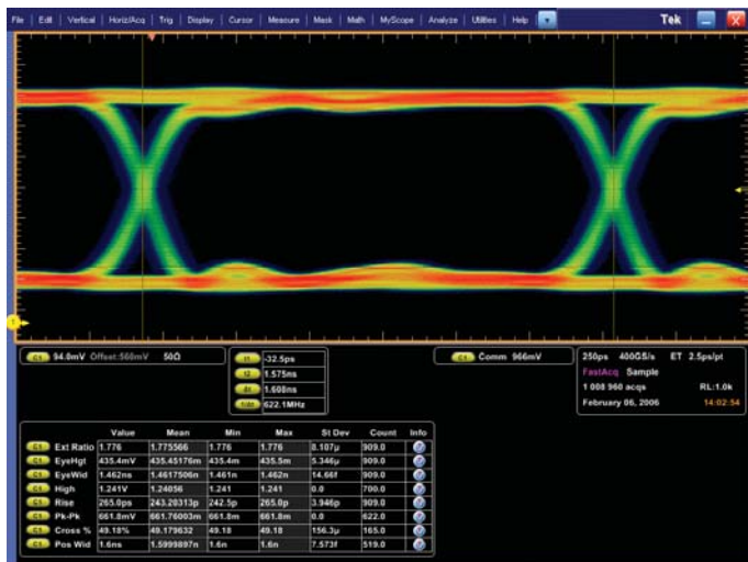
Figure 10a. 622 Mb/s serial data eye pattern.
