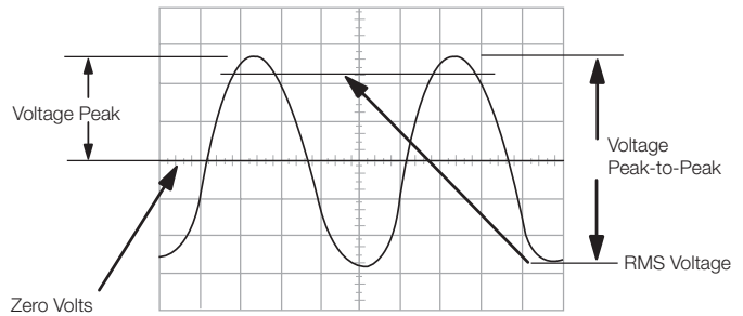
Figure 66. Voltage peak ( V_p ) and peak-to-peak voltage ( V_{p-p} )
