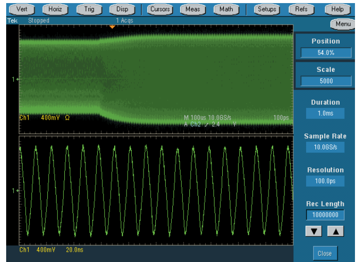
Figure 53. Capturing the high frequency detail of this modulated 85 MHz carrier requires high resolution sampling (100 ps). Seeing the signal's complete modulation envelope requires a long time duration (1 ms). Using long record length (10 MB), the oscilloscope can display both.
